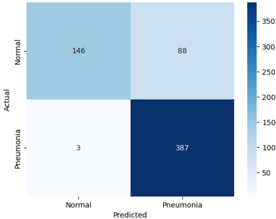
Confusion Matrix
